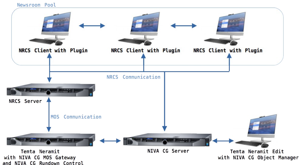
NIVA Temta Neramit with MOS Option Diagram
